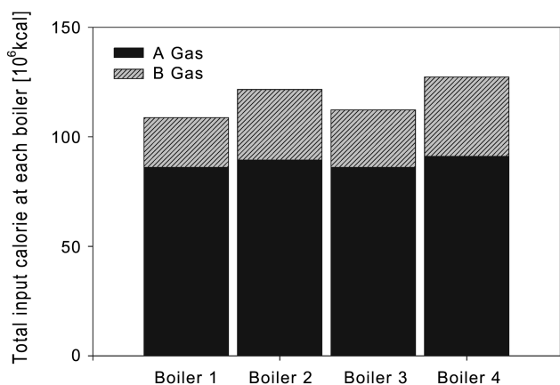
Fig. 10. Byproduct gas distribution result at period 3.
